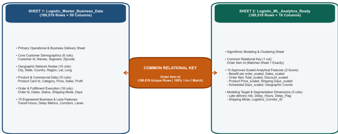
Figure 9: Professional Excel Workbook Dual-Sheet Relational Architecture & Analytical Separation
